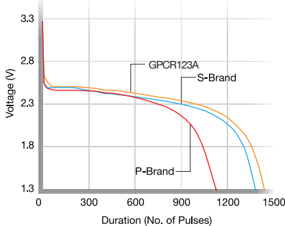
1200mA pulse discharge to 1.3V at 23°C
